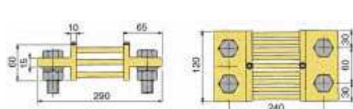
SH4000A/150mV (4,65Kg)
