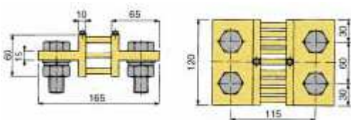
SH4000A/60mV (4,10Kg)
