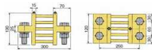
SH4000A/150mV (4,65Kg)
